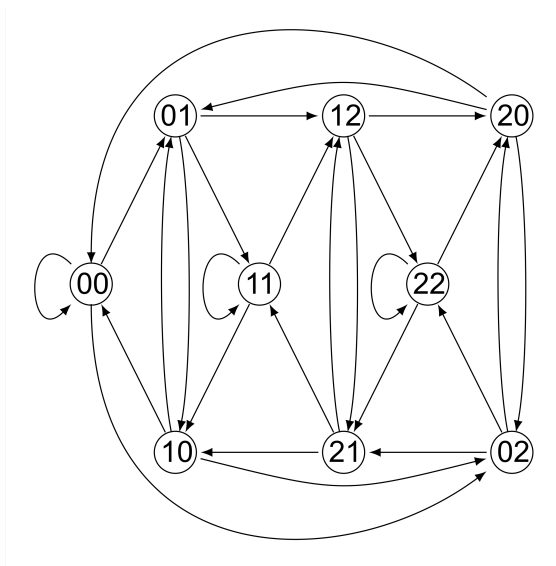
Figure 26.2 The De Bruijn graph B(3, 2) .
