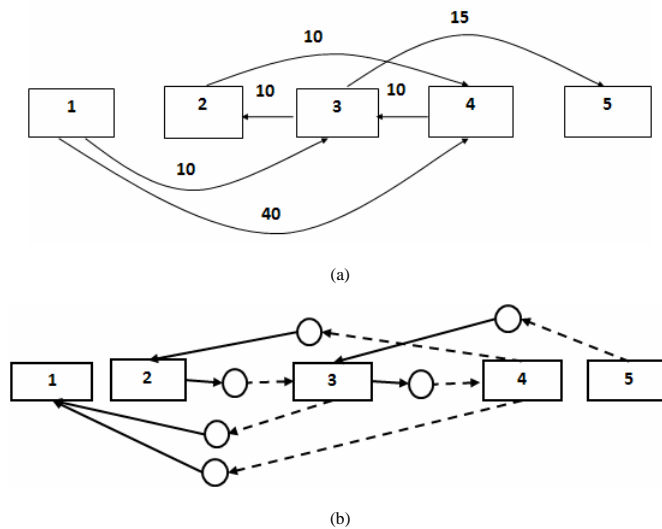
Figure 5: (a) Acyclic digraph; (b) Structural-dependencies d-graph; (c) Optimally weighted optimization-dependencies d-graph (bolded lines represent the arcs of the optimal-dependencies d-graph)
